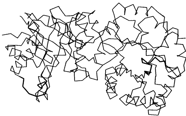
FIGURE 1 \alpha -Carbon trace of the crystal structure of the chicken TIM dimer. The two simulated flexible peptide loops are shown by bold lines in "open" conformations.
